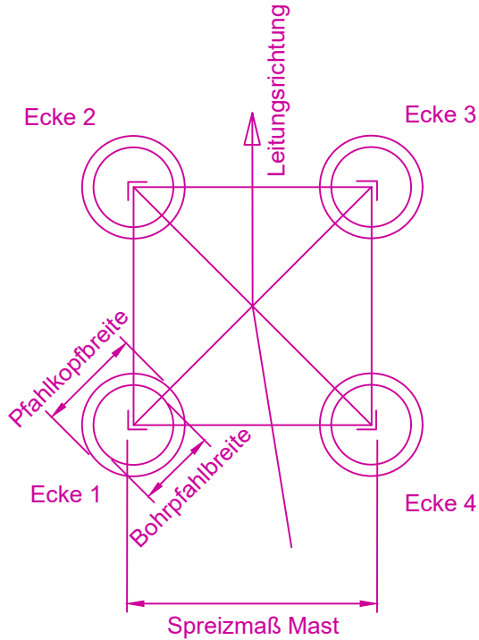
Grundriss (in Höhe EOK):
